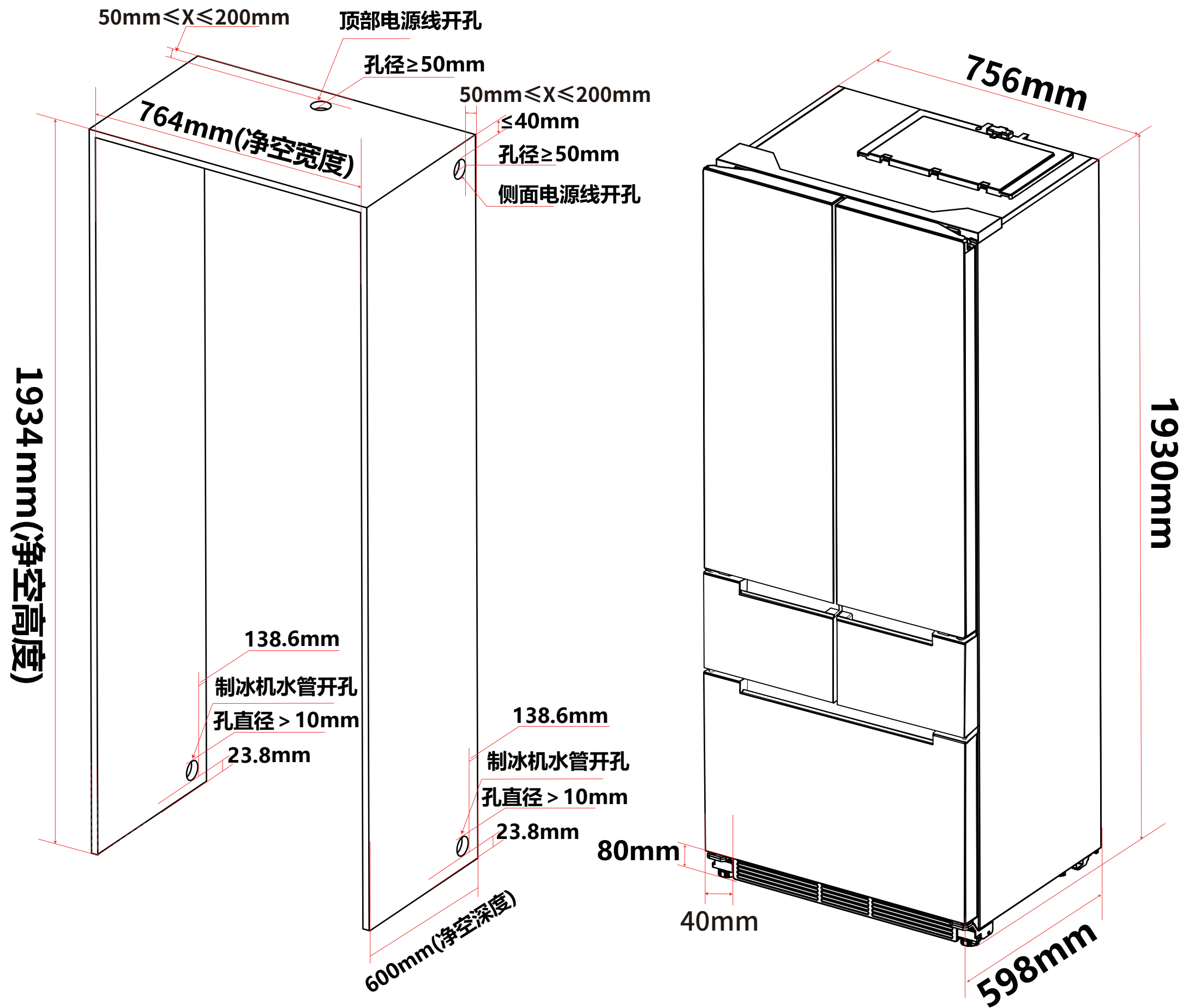
Traditional Mult door (平嵌五门)
